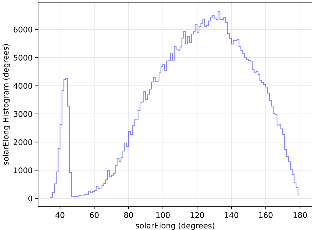
too_elab_r8_d2_ugrizy_v3.4_10yrs All sky z band: solarElong Histogram
