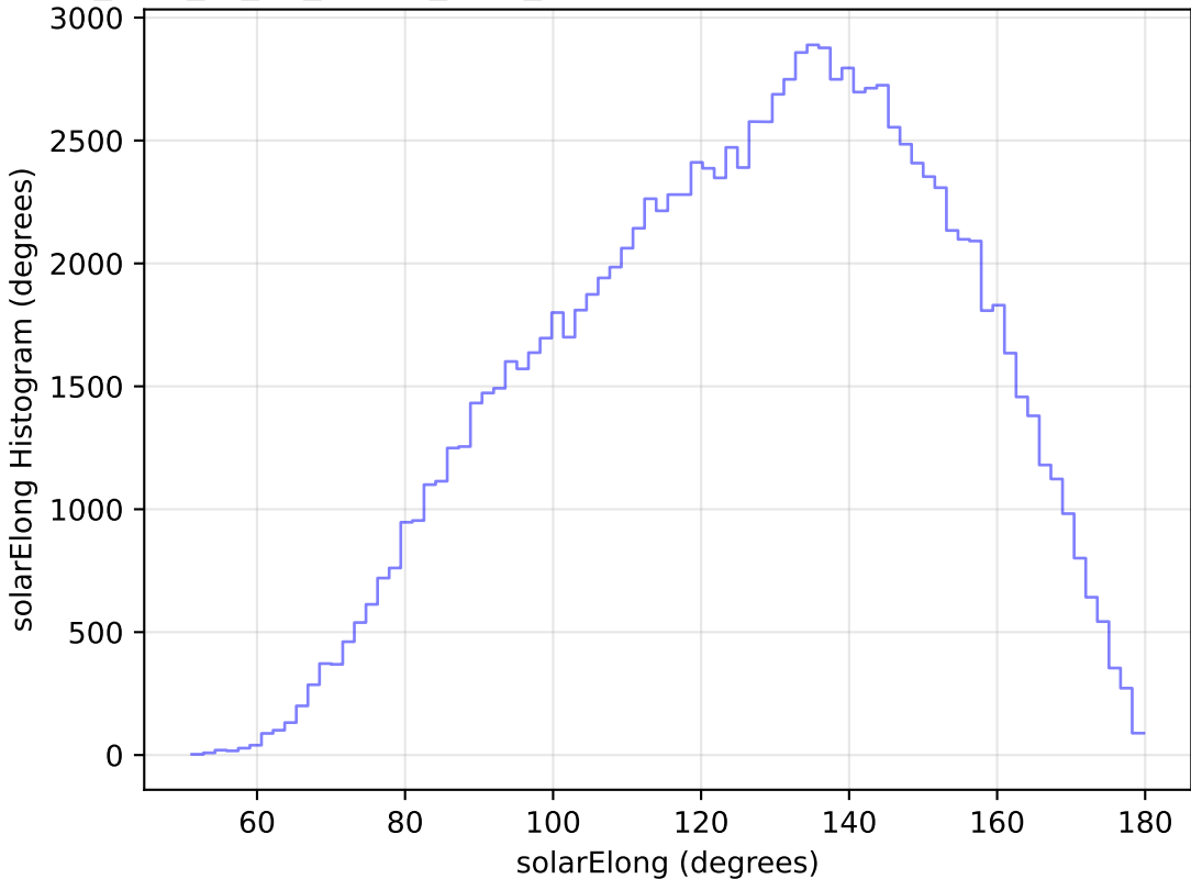
too_elab_r8_d2_ugrizy_v3.4_10yrs All sky u band: solarElong Histogram
