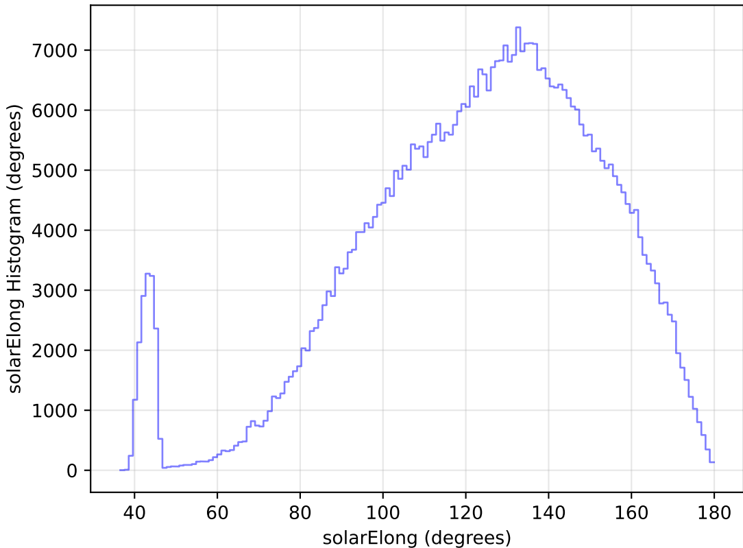
too_elab_r8_d2_ugrizy_v3.4_10yrs All sky r band: solarElong Histogram
