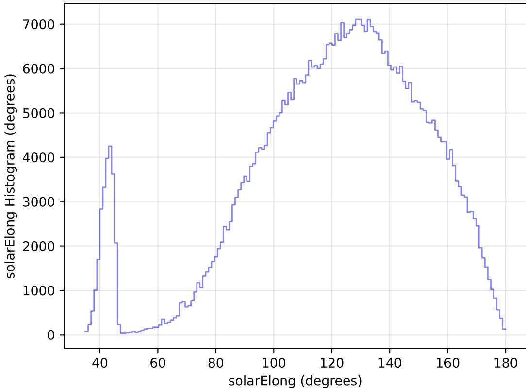
too_elab_r8_d2_ugrizy_v3.4_10yrs All sky i band: solarElong Histogram
