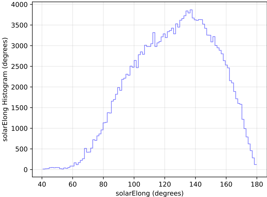
too_elab_r8_d2_ugrizy_v3.4_10yrs All sky g band: solarElong Histogram
