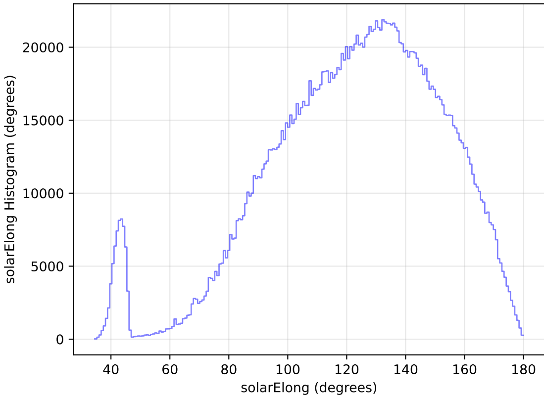
too_elab_r8_d2_ugrizy_v3.4_10yrs All sky all bands: solarElong Histogram
