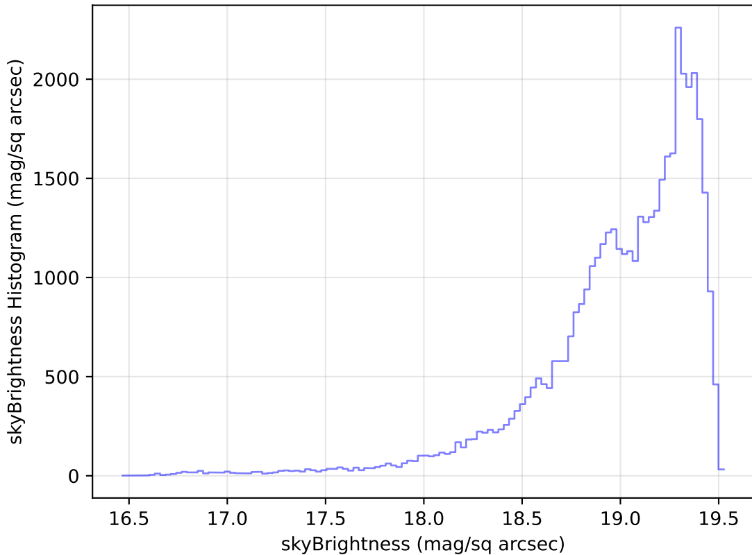
too_elab_r8_d2_ugrizy_v3.4_10yrs Yr 1 z band: skyBrightness Histogram
