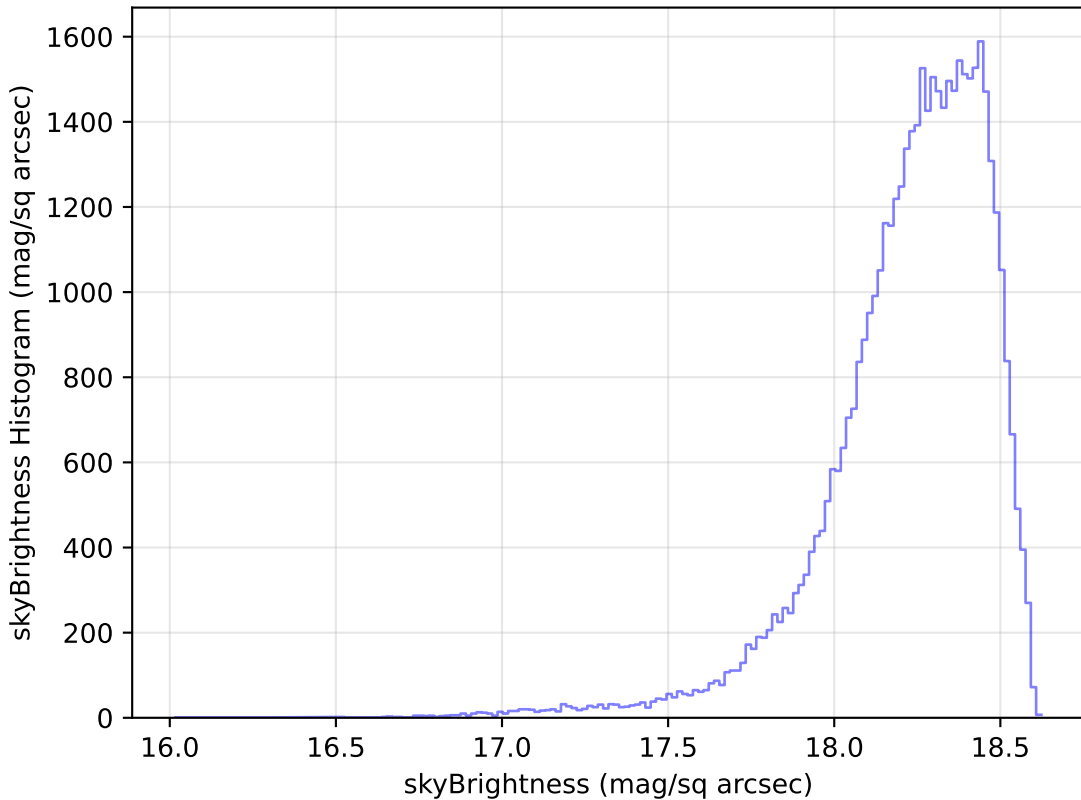
too_elab_r8_d2_ugrizy_v3.4_10yrs Yr 1 y band: skyBrightness Histogram
