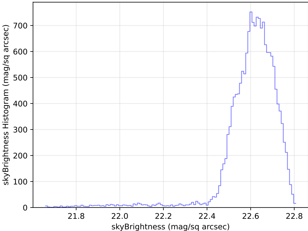
too_elab_r8_d2_ugrizy_v3.4_10yrs Yr 1 u band: skyBrightness Histogram
