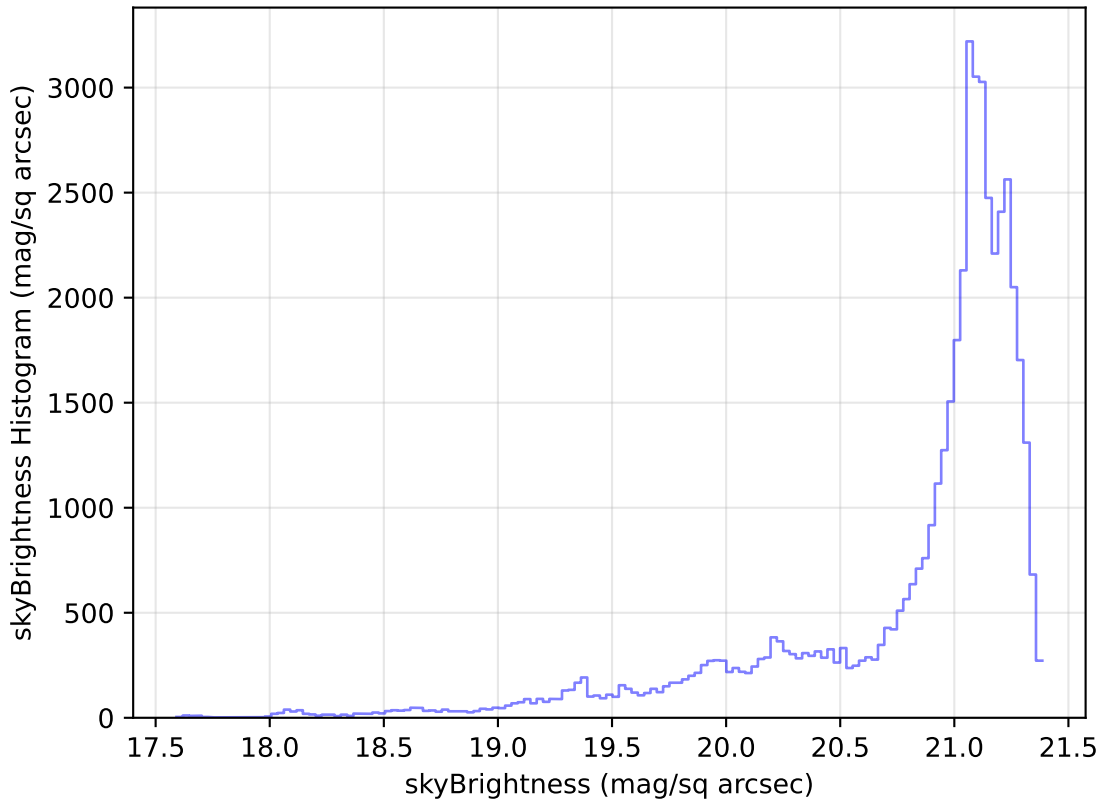
too_elab_r8_d2_ugrizy_v3.4_10yrs Yr 1 r band: skyBrightness Histogram
