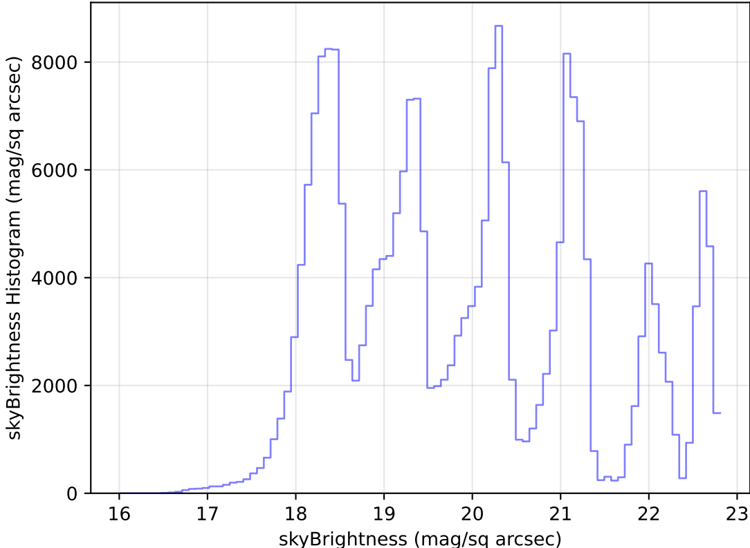
too_elab_r8_d2_ugrizy_v3.4_10yrs Yr 1 all bands: skyBrightness Histogram
