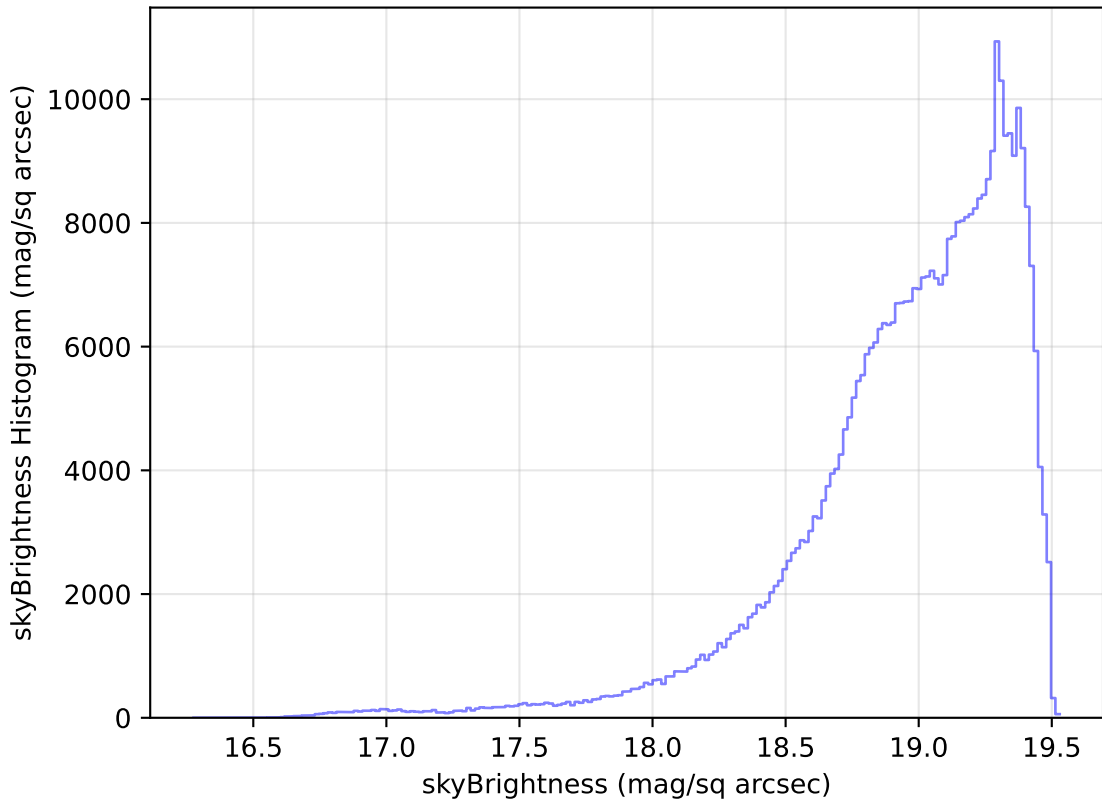
too_elab_r8_d2_ugrizy_v3.4_10yrs WFD z band: skyBrightness Histogram
