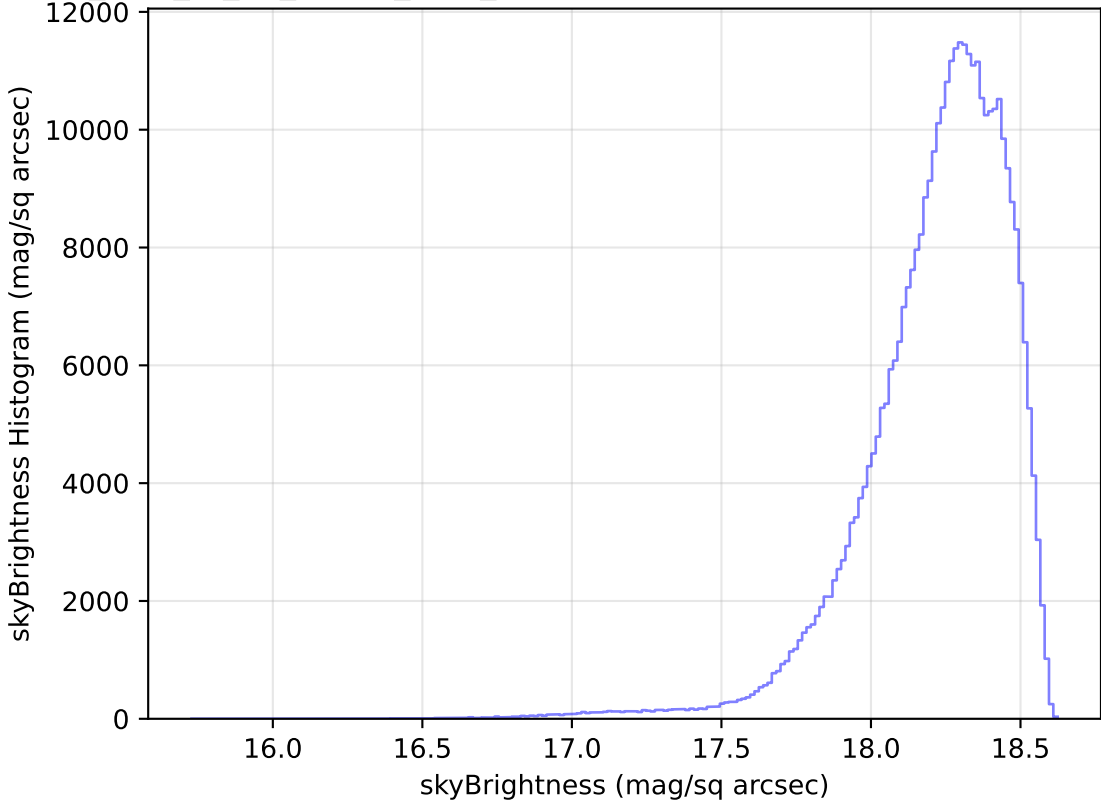
too_elab_r8_d2_ugrizy_v3.4_10yrs WFD y band: skyBrightness Histogram
