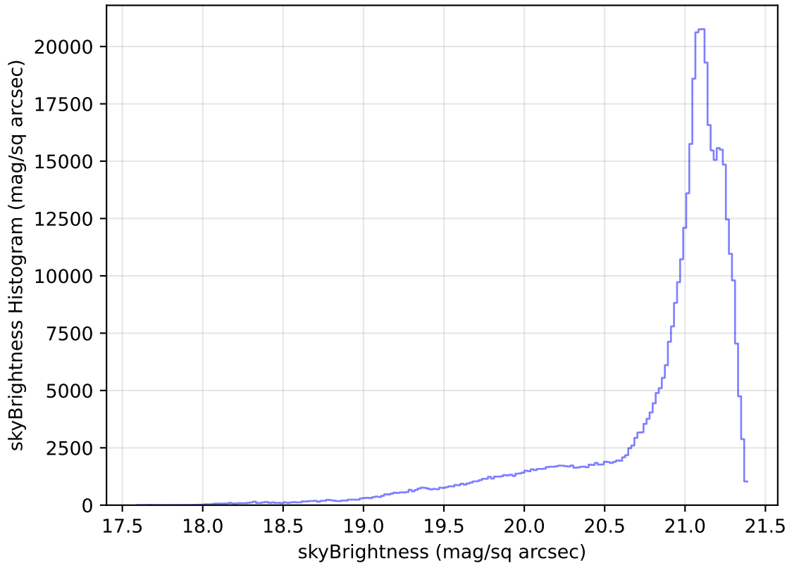
too_elab_r8_d2_ugrizy_v3.4_10yrs WFD r band: skyBrightness Histogram
