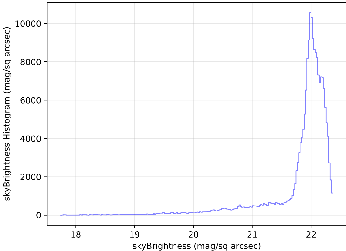
too_elab_r8_d2_ugrizy_v3.4_10yrs WFD g band: skyBrightness Histogram
