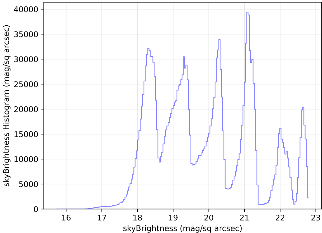
too_elab_r8_d2_ugrizy_v3.4_10yrs WFD all bands: skyBrightness Histogram
