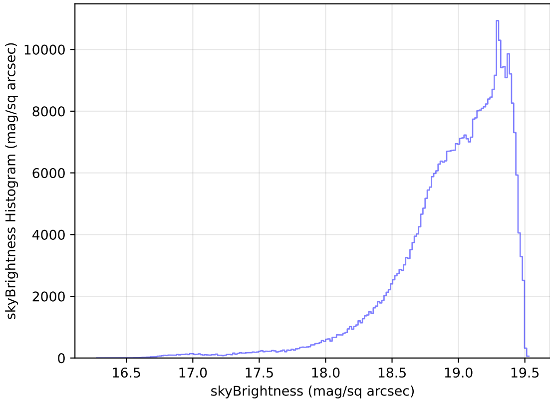
too_elab_r8_d2_ugrizy_v3.4_10yrs All sky z band: skyBrightness Histogram
