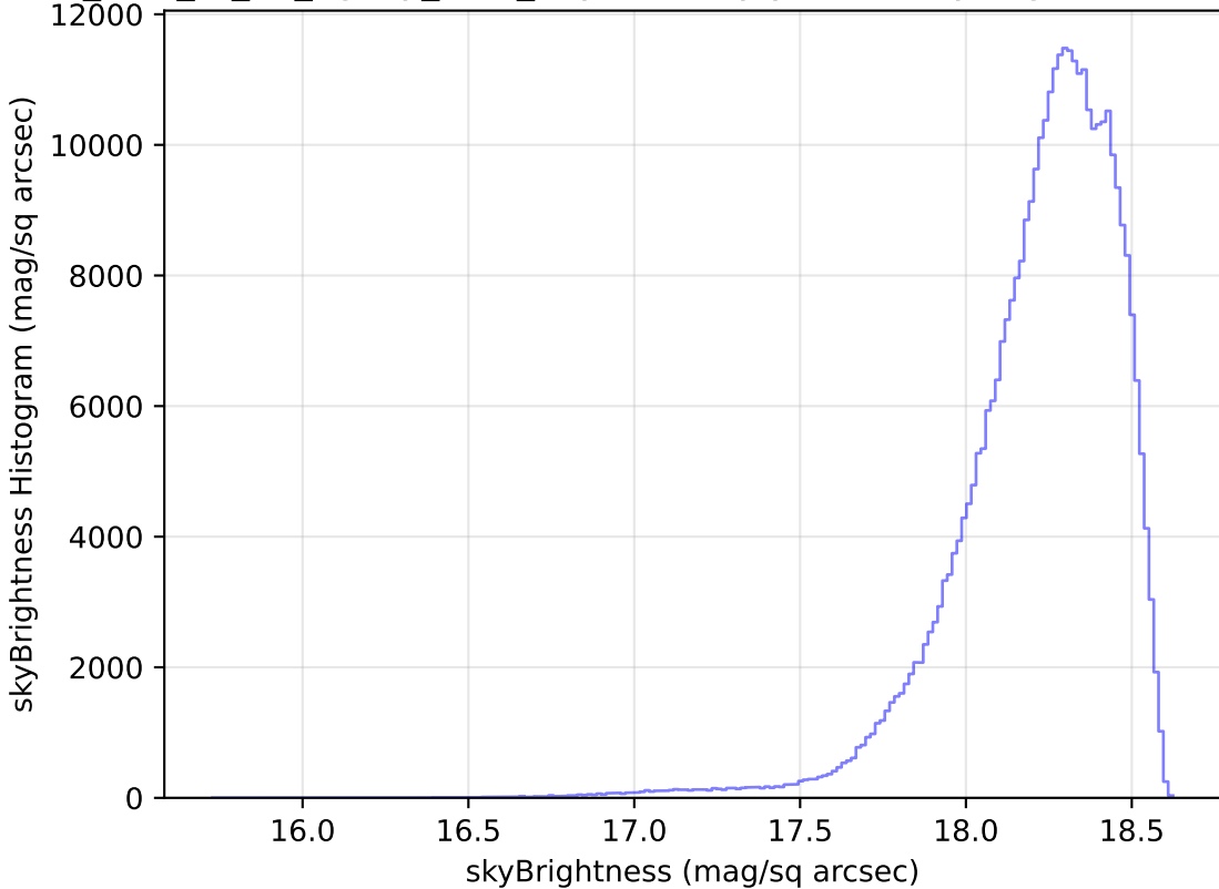
too_elab_r8_d2_ugrizy_v3.4_10yrs All sky y band: skyBrightness Histogram
