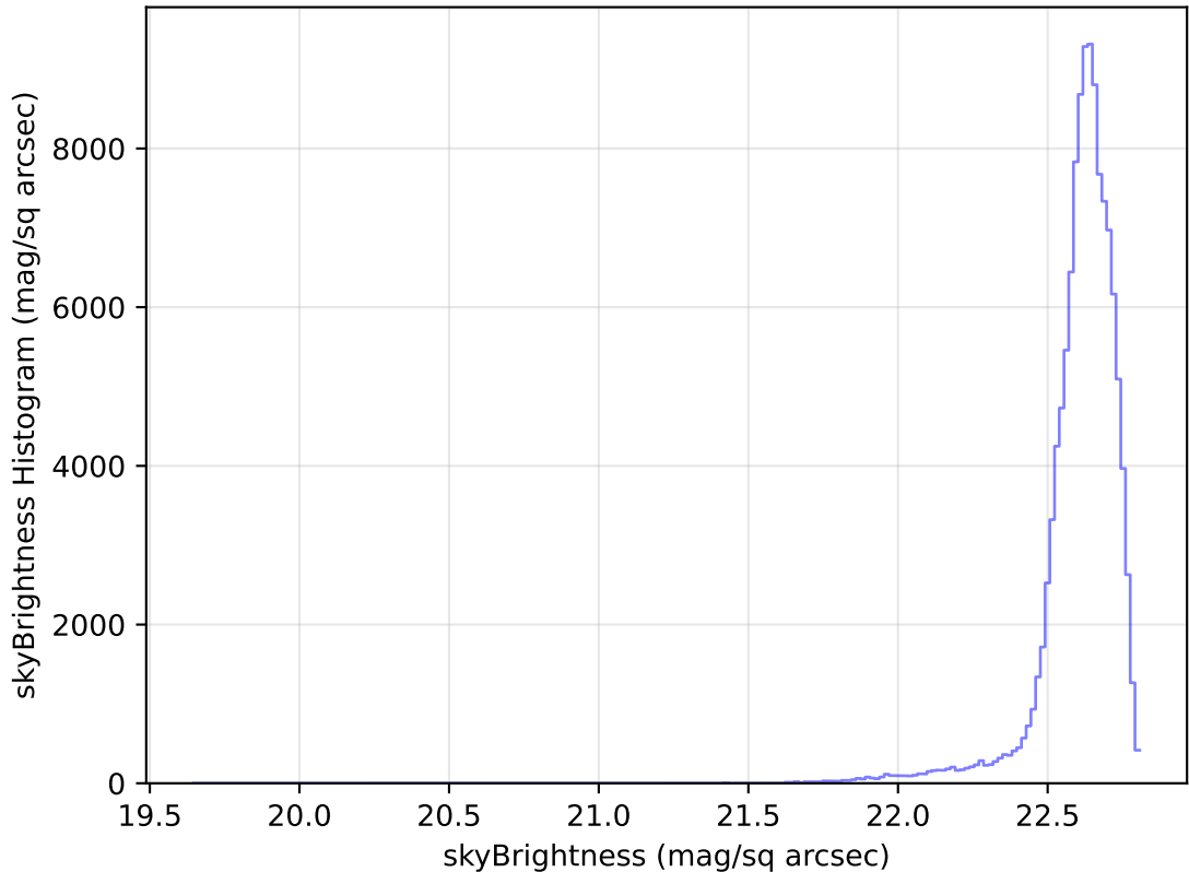
too_elab_r8_d2_ugrizy_v3.4_10yrs All sky u band: skyBrightness Histogram
