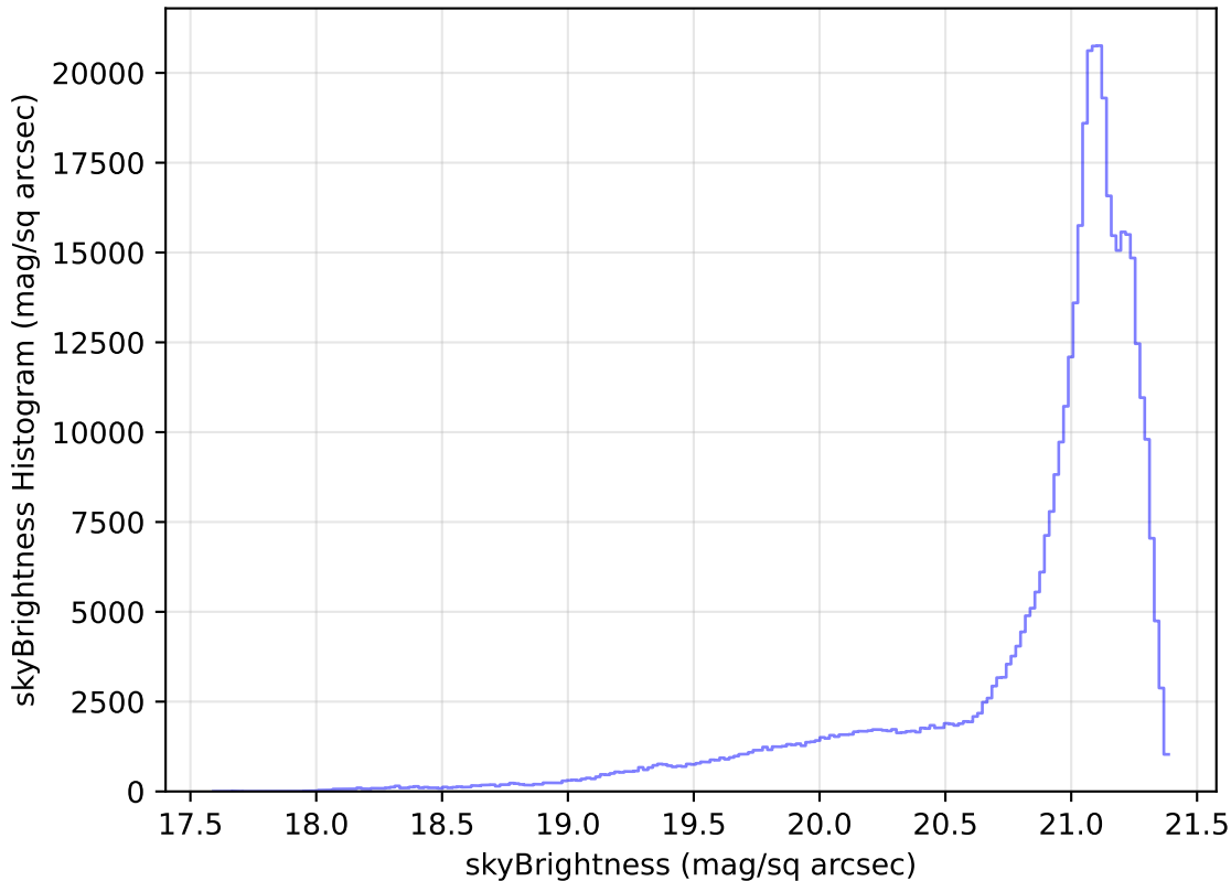
too_elab_r8_d2_ugrizy_v3.4_10yrs All sky r band: skyBrightness Histogram
