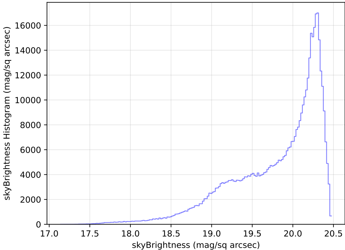
too_elab_r8_d2_ugrizy_v3.4_10yrs All sky i band: skyBrightness Histogram
