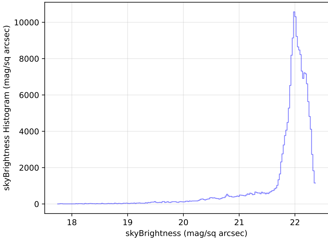
too_elab_r8_d2_ugrizy_v3.4_10yrs All sky g band: skyBrightness Histogram
