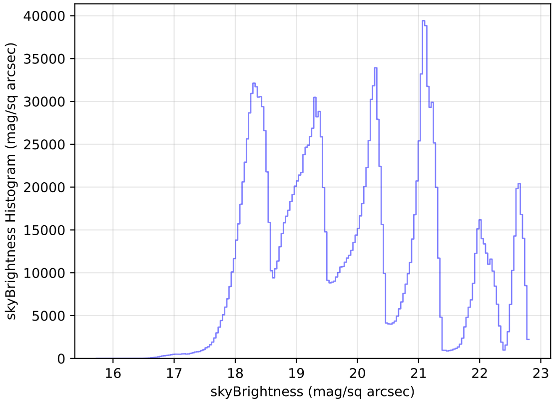
too_elab_r8_d2_ugrizy_v3.4_10yrs All sky all bands: skyBrightness Histogram
