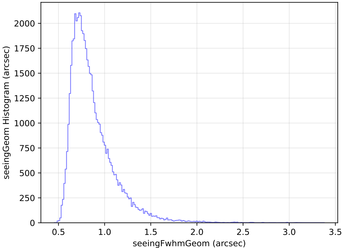
too_elab_r8_d2_ugrizy_v3.4_10yrs Yr 1 i band: seeingGeom Histogram
