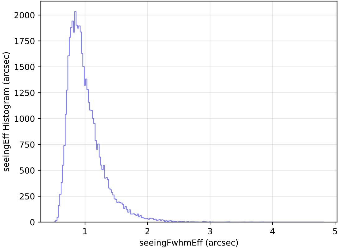
too_elab_r8_d2_ugrizy_v3.4_10yrs Yr 1 z band: seeingEff Histogram
