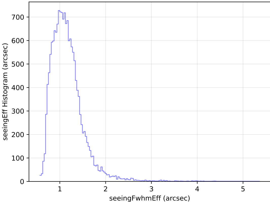
too_elab_r8_d2_ugrizy_v3.4_10yrs Yr 1 u band: seeingEff Histogram
