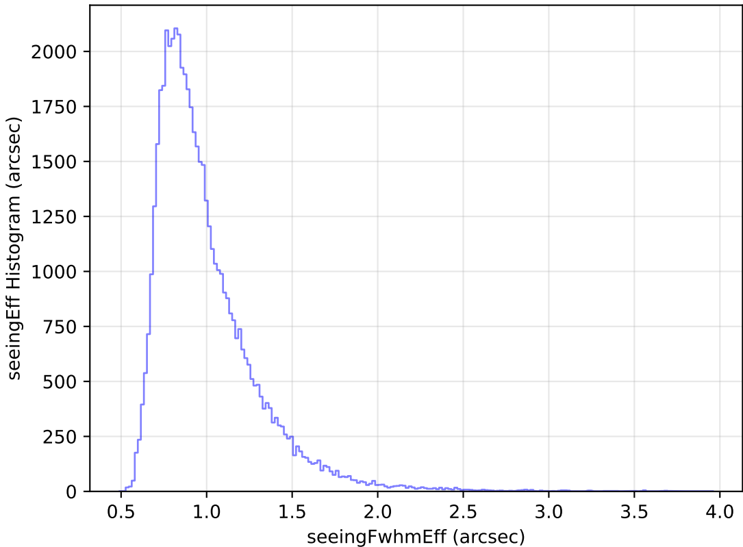
too_elab_r8_d2_ugrizy_v3.4_10yrs Yr 1 i band: seeingEff Histogram
