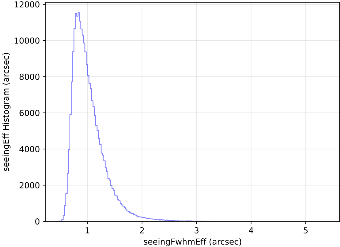
too_elab_r8_d2_ugrizy_v3.4_10yrs Yr 1 all bands: seeingEff Histogram
