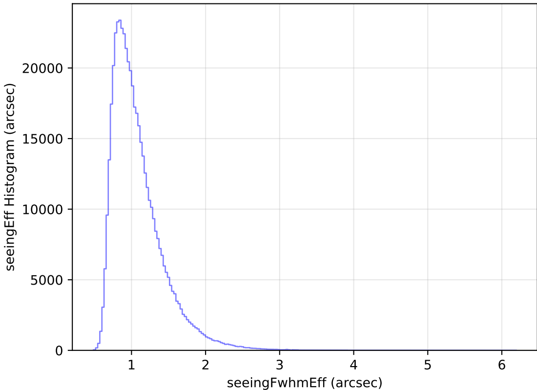
too_elab_r8_d2_ugrizy_v3.4_10yrs WFD i band: seeingEff Histogram
