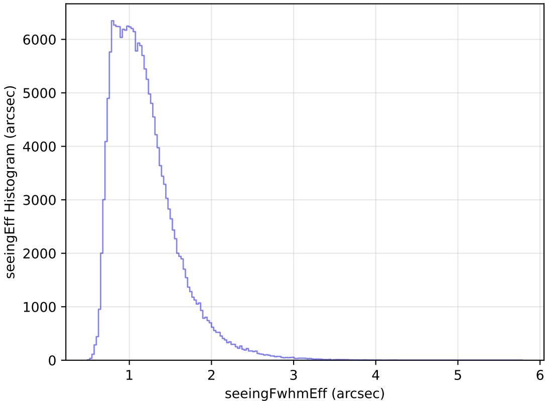
too_elab_r8_d2_ugrizy_v3.4_10yrs WFD g band: seeingEff Histogram
