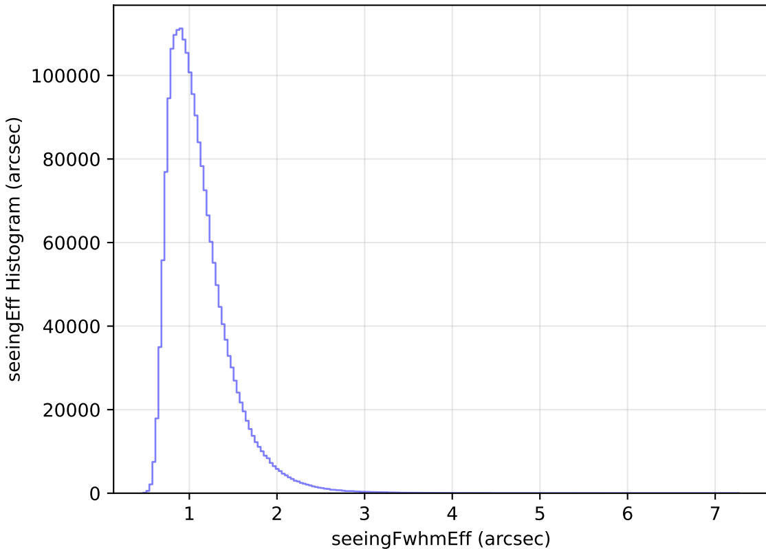
too_elab_r8_d2_ugrizy_v3.4_10yrs WFD all bands: seeingEff Histogram
