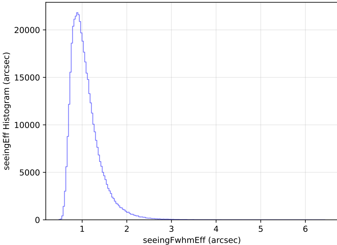
too_elab_r8_d2_ugrizy_v3.4_10yrs All sky z band: seeingEff Histogram
