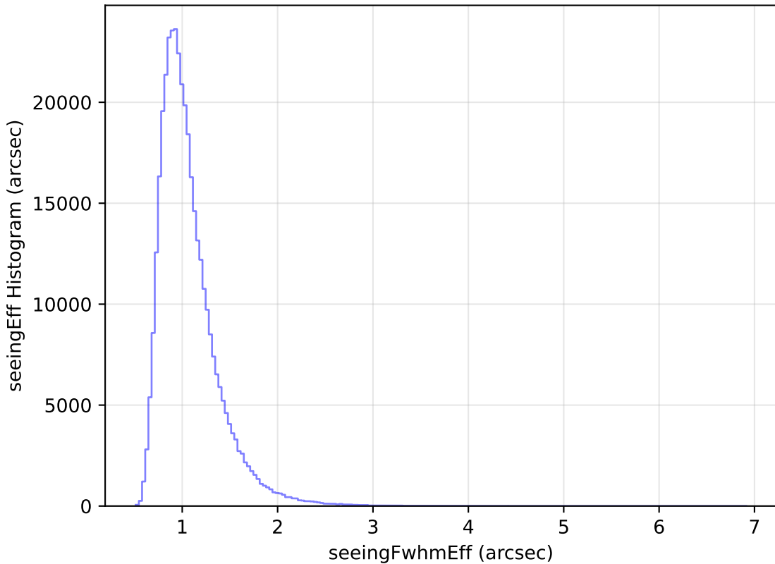
too_elab_r8_d2_ugrizy_v3.4_10yrs All sky y band: seeingEff Histogram
