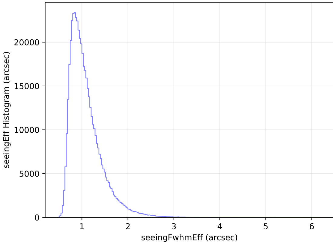
too_elab_r8_d2_ugrizy_v3.4_10yrs All sky i band: seeingEff Histogram
