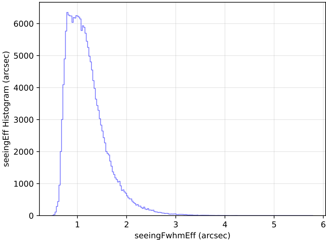
too_elab_r8_d2_ugrizy_v3.4_10yrs All sky g band: seeingEff Histogram
