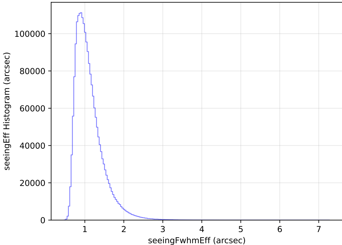
too_elab_r8_d2_ugrizy_v3.4_10yrs All sky all bands: seeingEff Histogram
