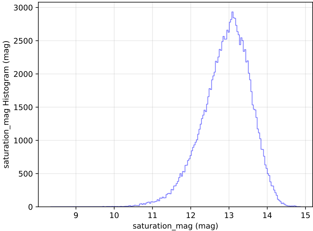
too_elab_r8_d2_ugrizy_v3.4_10yrs WFD u band: saturation_mag Histogram
