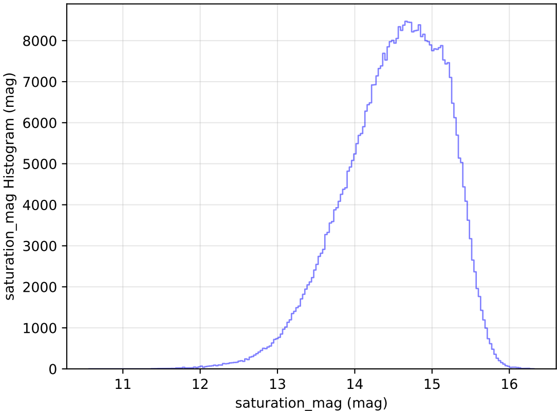
too_elab_r8_d2_ugrizy_v3.4_10yrs WFD r band: saturation_mag Histogram
