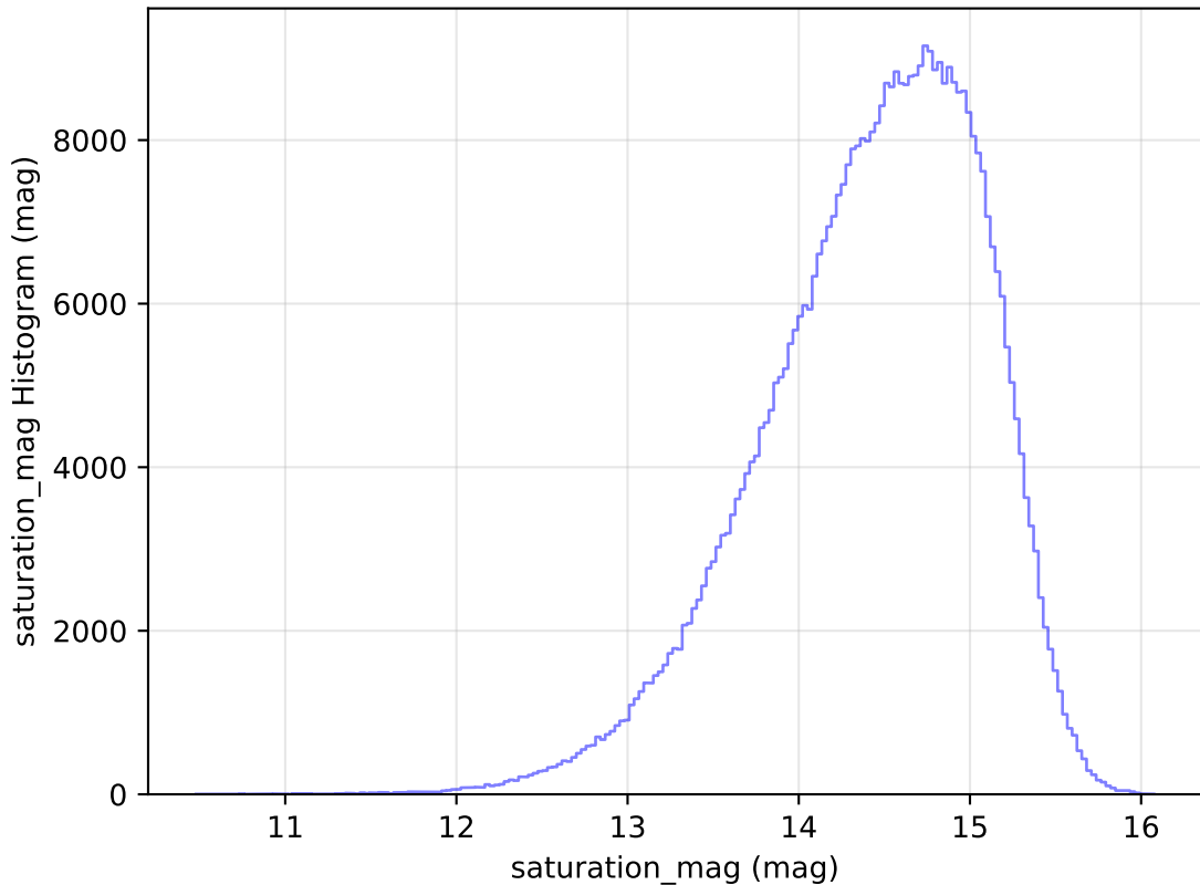
too_elab_r8_d2_ugrizy_v3.4_10yrs WFD i band: saturation_mag Histogram
