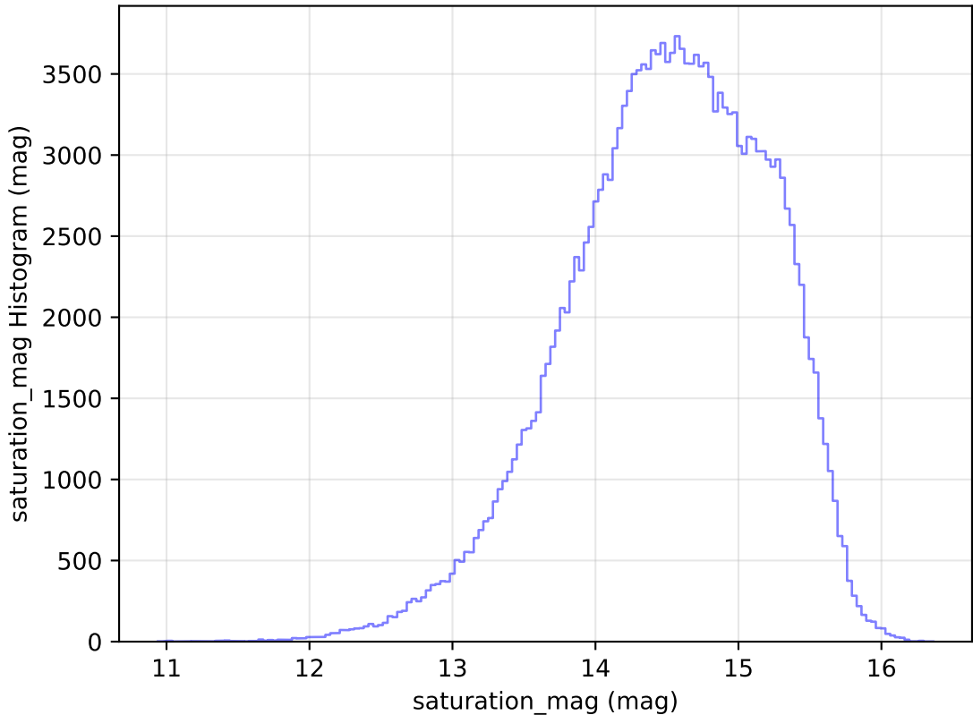
too_elab_r8_d2_ugrizy_v3.4_10yrs WFD g band: saturation_mag Histogram
