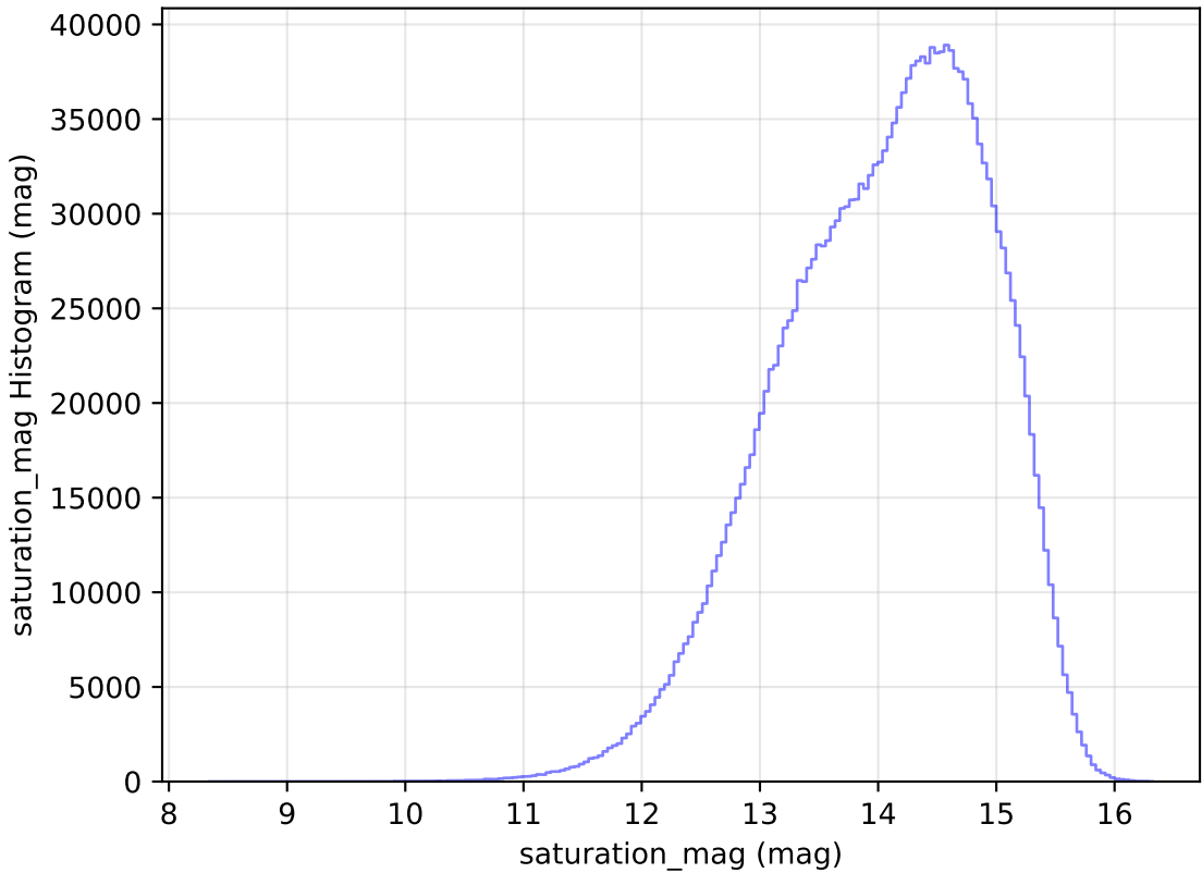
too_elab_r8_d2_ugrizy_v3.4_10yrs WFD all bands: saturation_mag Histogram
