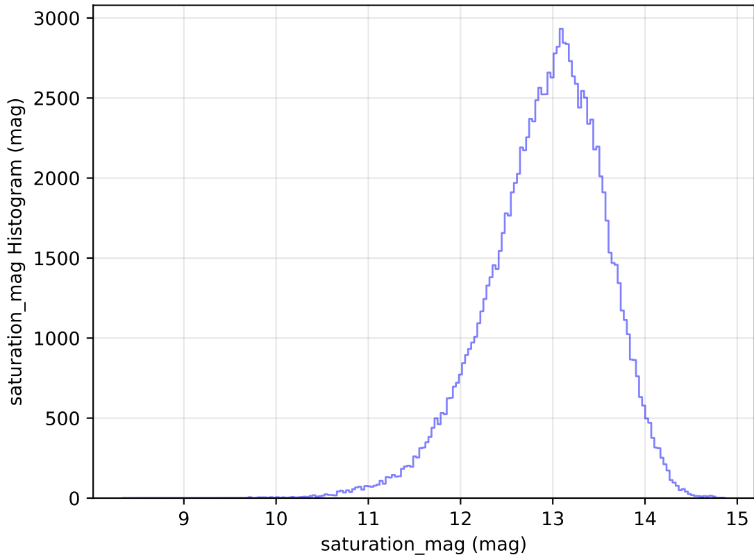
too_elab_r8_d2_ugrizy_v3.4_10yrs All sky u band: saturation_mag Histogram
