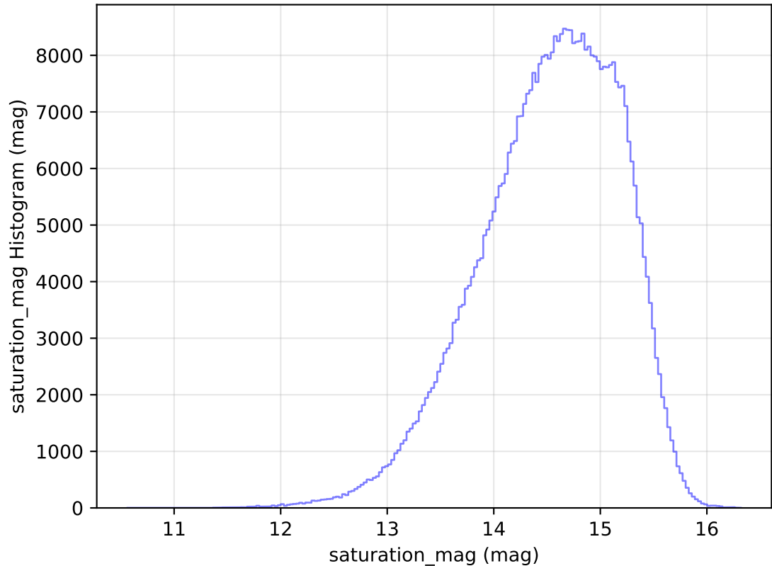
too_elab_r8_d2_ugrizy_v3.4_10yrs All sky r band: saturation_mag Histogram
