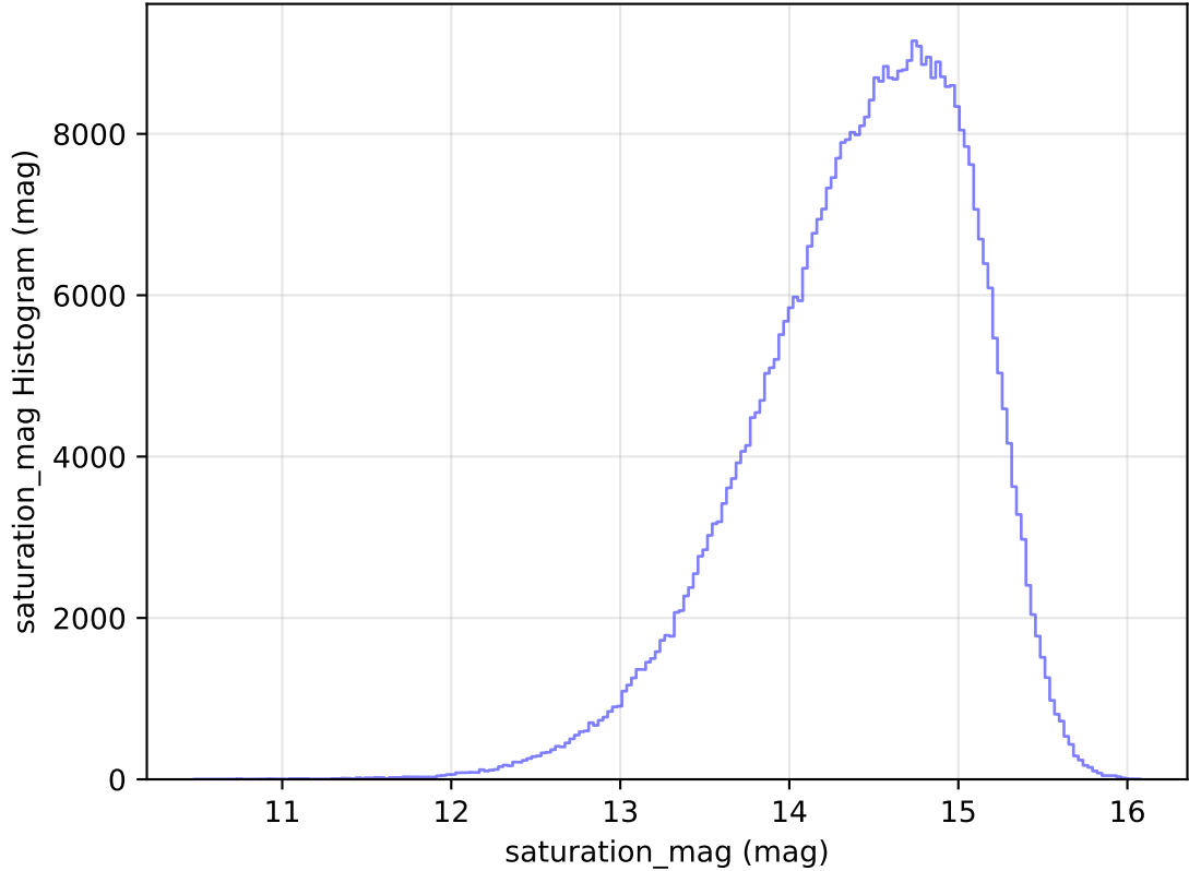
too_elab_r8_d2_ugrizy_v3.4_10yrs All sky i band: saturation_mag Histogram
