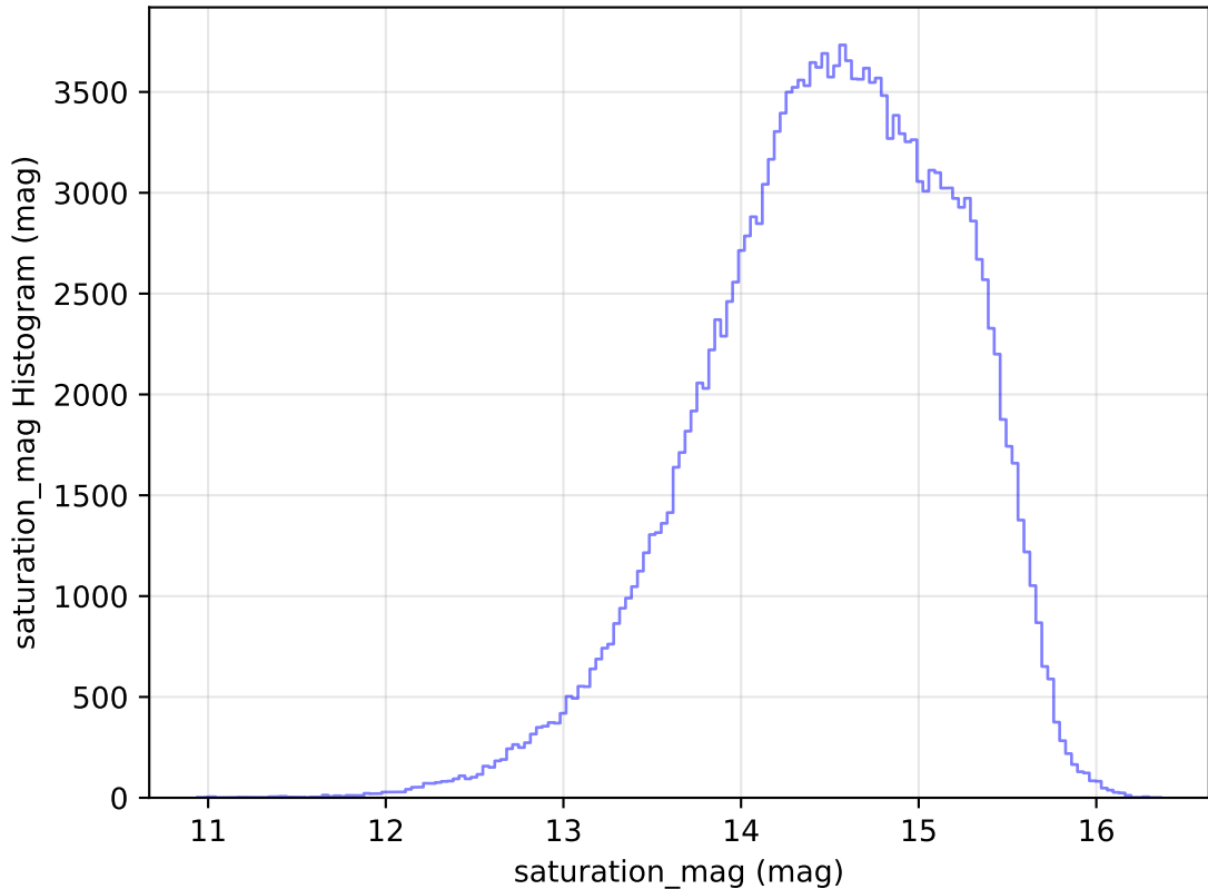
too_elab_r8_d2_ugrizy_v3.4_10yrs All sky g band: saturation_mag Histogram
