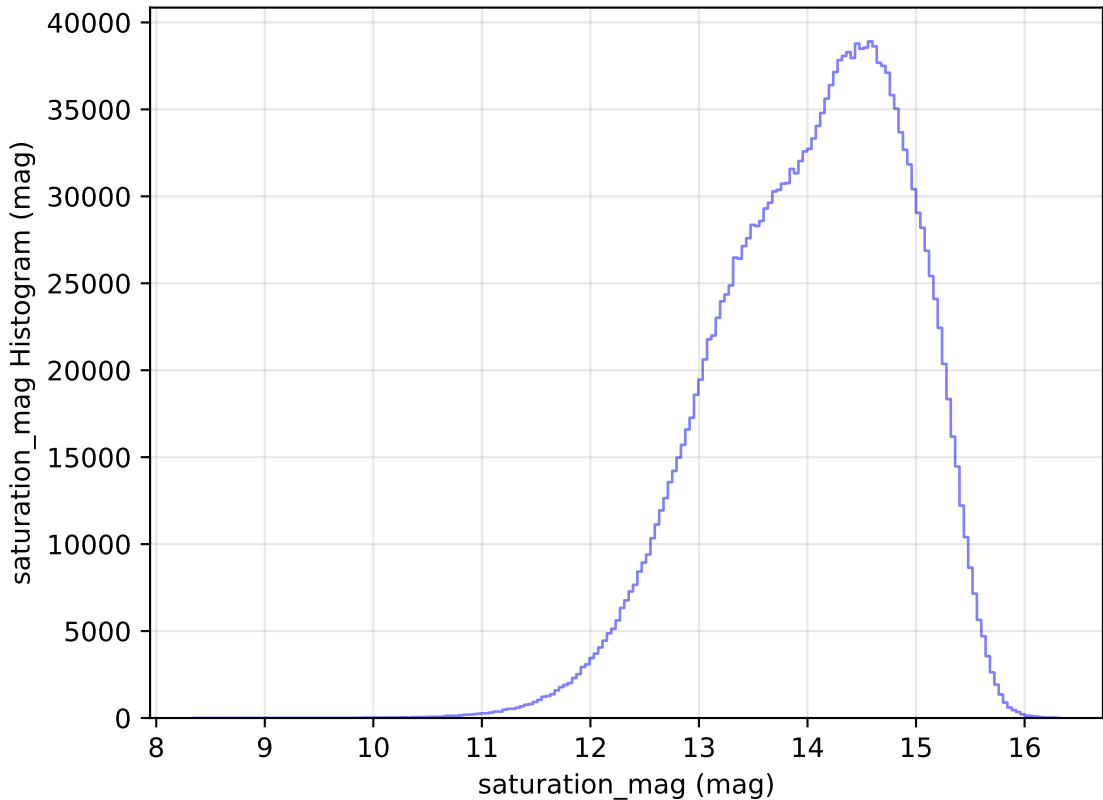
too_elab_r8_d2_ugrizy_v3.4_10yrs All sky all bands: saturation_mag Histogram
