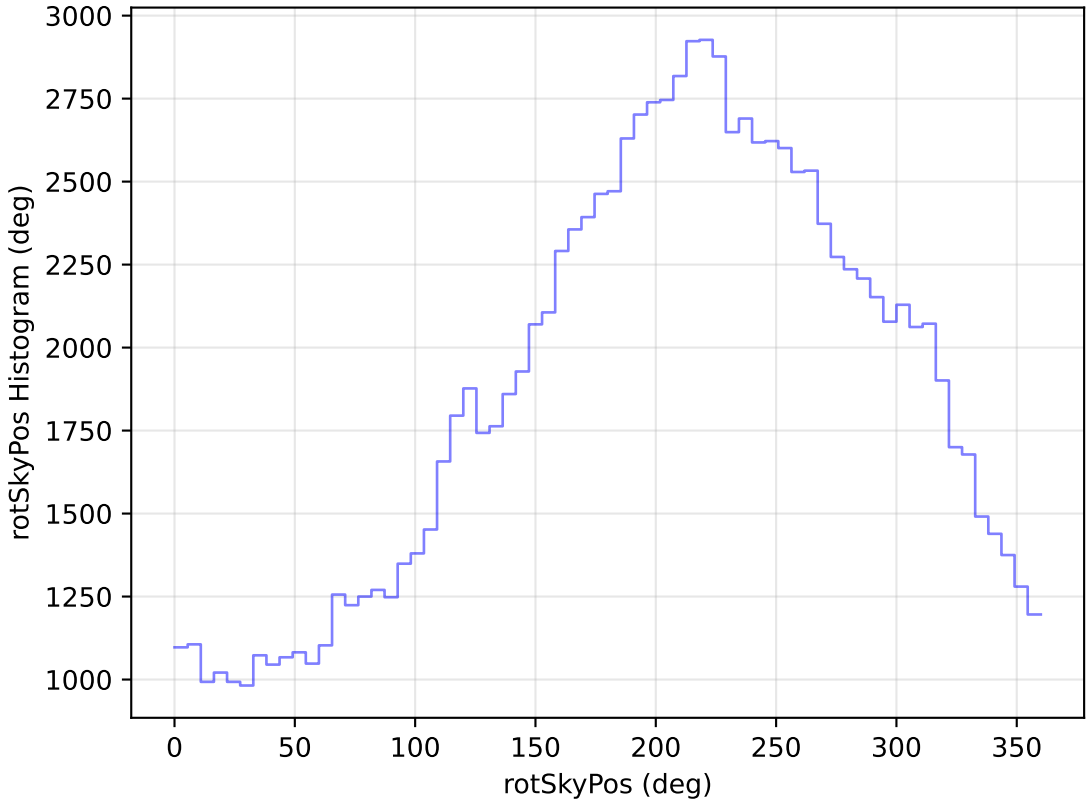
too_elab_r8_d2_ugrizy_v3.4_10yrs WFD u band: rotSkyPos Histogram
