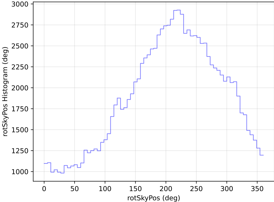
too_elab_r8_d2_ugrizy_v3.4_10yrs All sky u band: rotSkyPos Histogram
