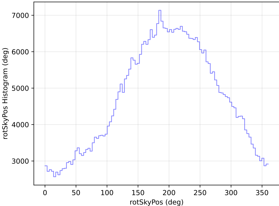
too_elab_r8_d2_ugrizy_v3.4_10yrs All sky r band: rotSkyPos Histogram
