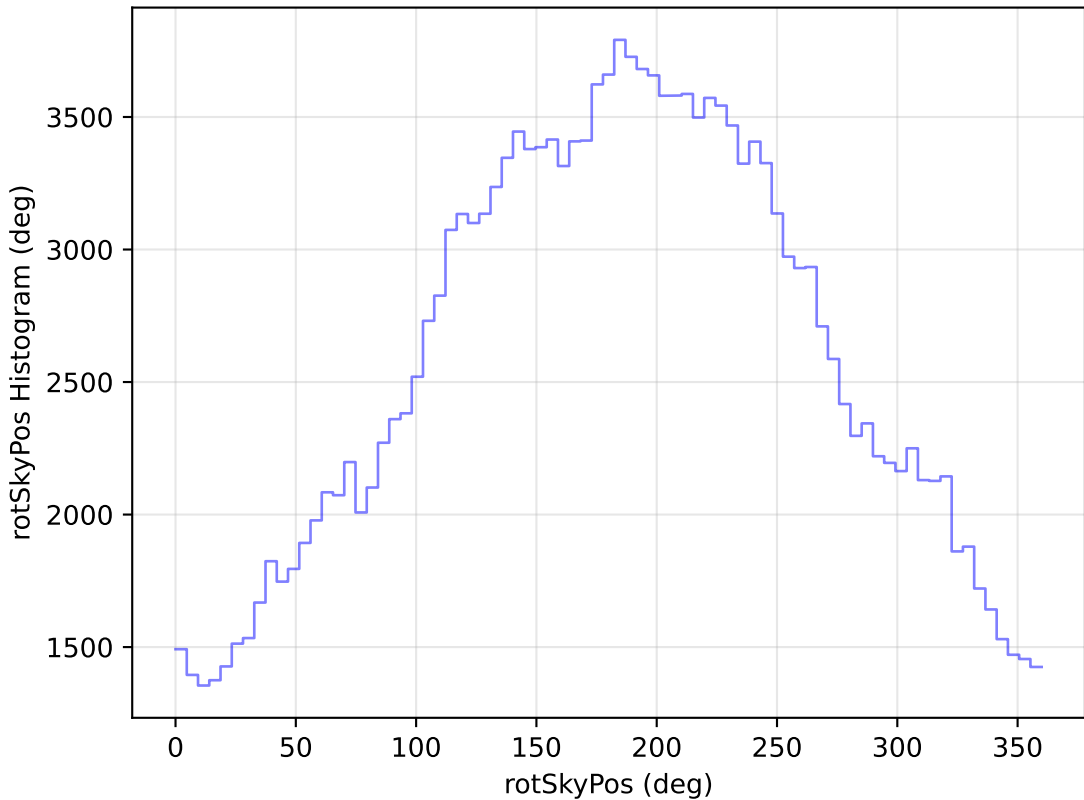
too_elab_r8_d2_ugrizy_v3.4_10yrs All sky g band: rotSkyPos Histogram
